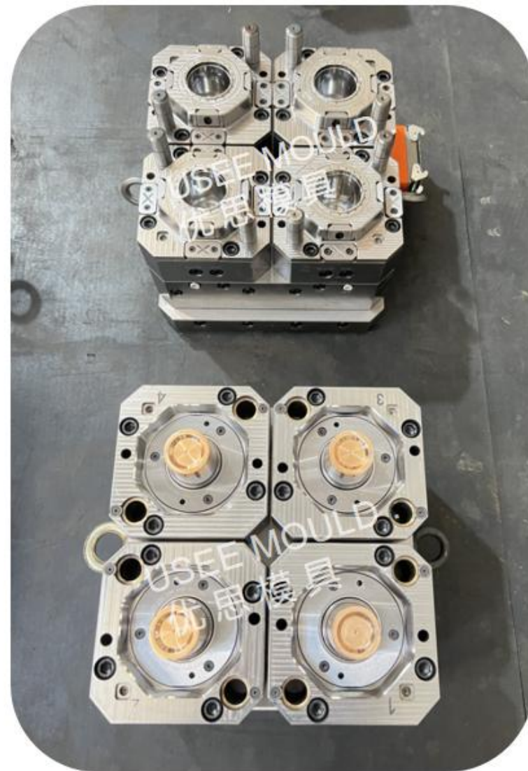
250 ML bucket mould
