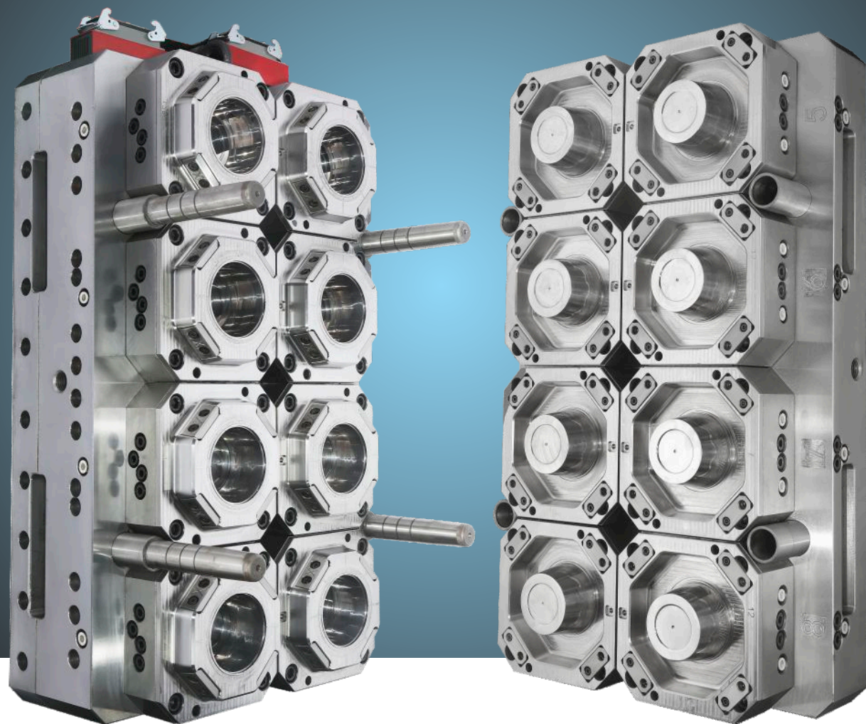
Mould Name: thin wall container mould Plastic Material: PP Cavities No.: 8 Cavities Volume: 475ml Part Weight: Container 10 g Lid 6 g Runner Type: full hot runner Mould Steel: 2344
