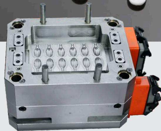
Mould Name: Fold fork mould Plastic Material: PP Cavities No.: 12 Cavities Part Weight: 1.95g Runner Type: Full hot runner Mould Steel: S136
